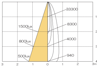
ELA-100HCW25
