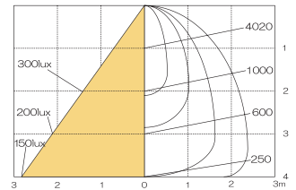
ELA-100HCW80
