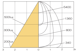
ELA-100HCW60
